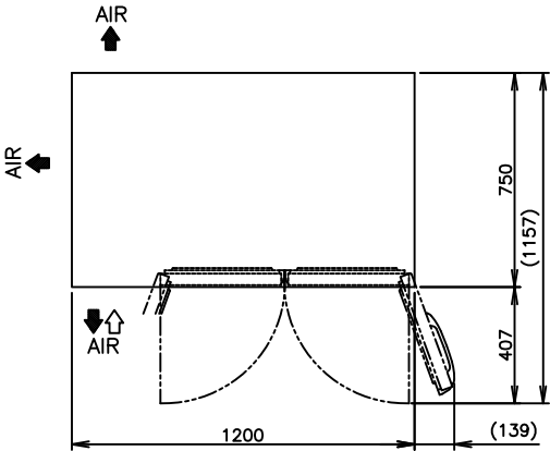
VIEW A
